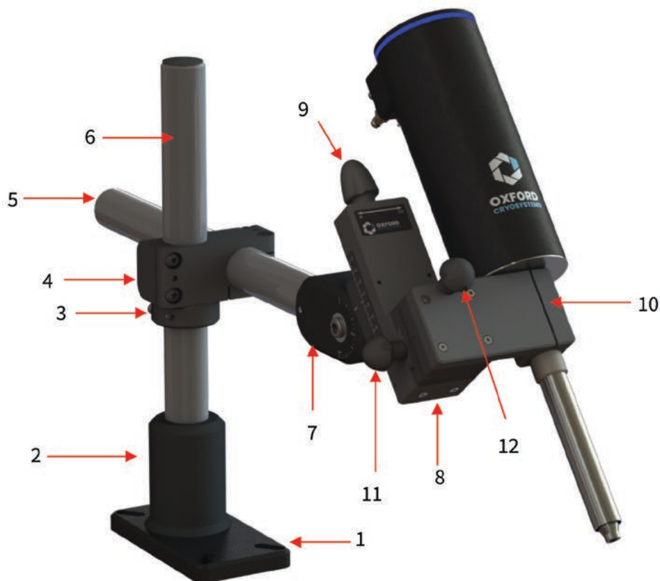
Figure 6.2 The principal components within the assembly
