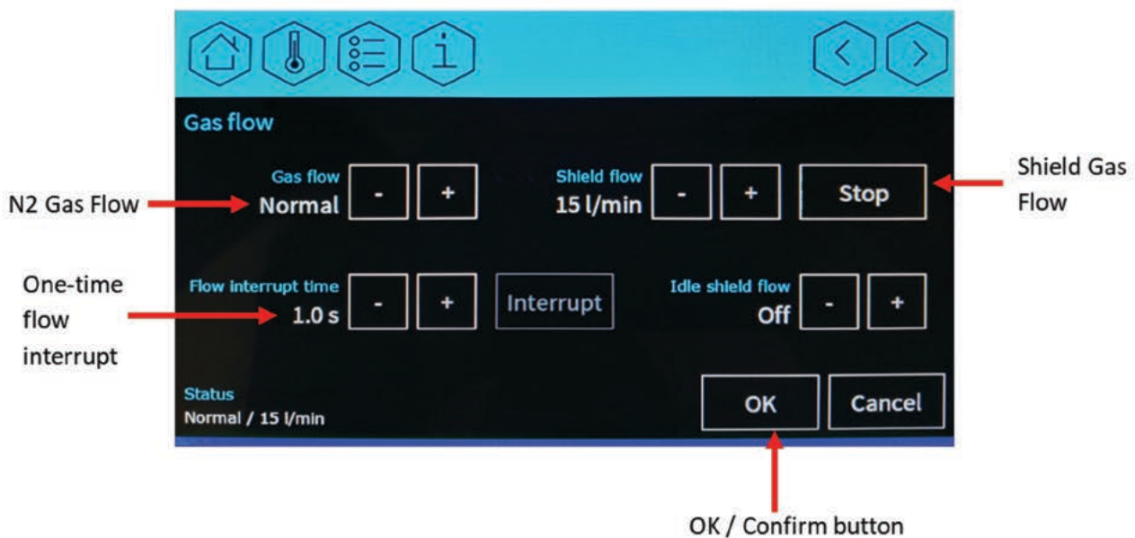
Figure 7.12 Command screen 2 showing gas flow settings
