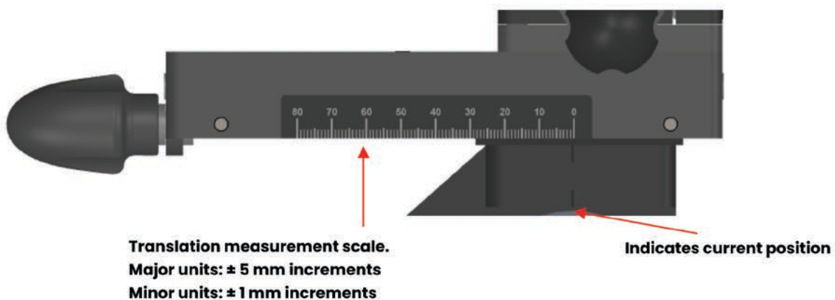
Figure 6.5 Varibeam Adjustment points
